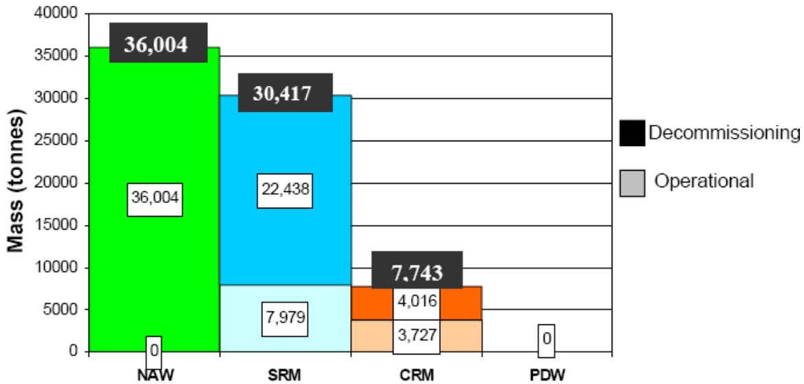
Figure 3 : Material masses after 100 years of shutdown of power plant conceptual study model B. Extracted from [2]. NAW is Non Active Waste, SRM is Simple Recycle Material, CRM is Complex Recycle Material, and PDW is Permanent Disposal Waste (non-recyclable).
